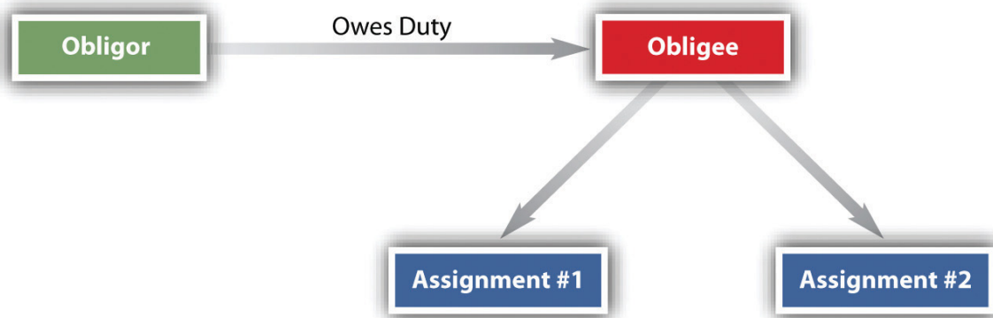
Figure 14.2 Successive Assignments
