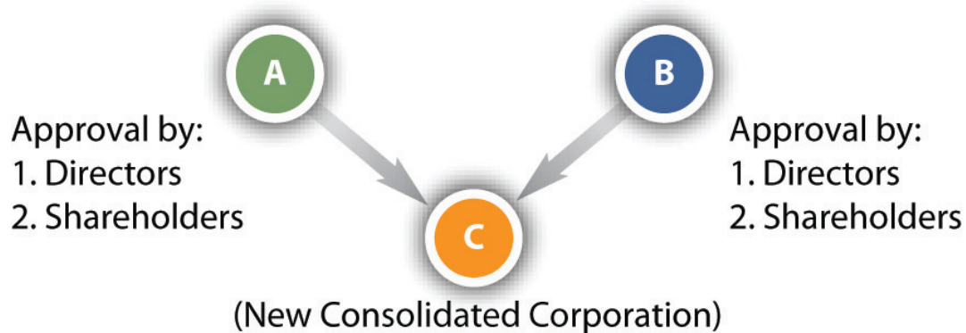
Figure 27.3 Consolidation
