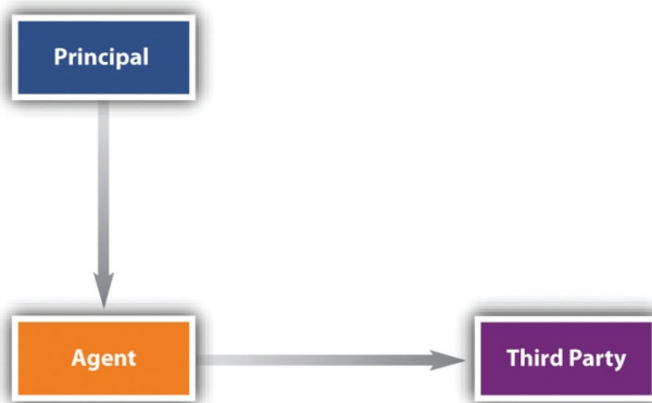
Figure 18.1 Agency Relationships
